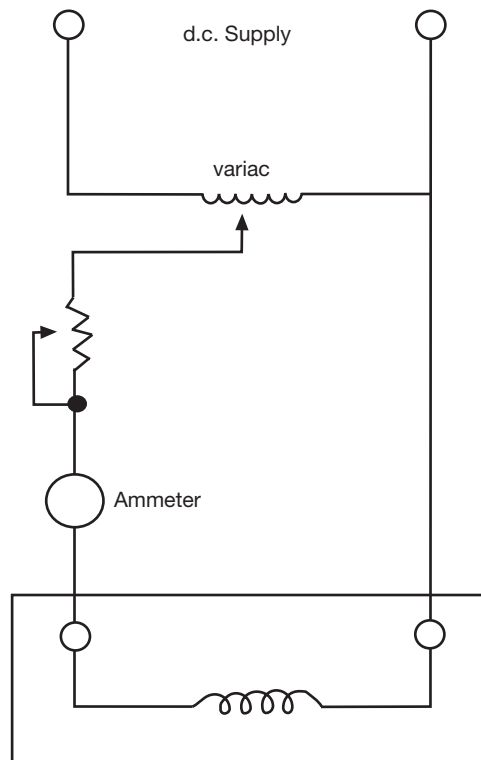
Fig. 7b Secondary injection test of guard relays. (Refer to relevent schematic for terminal nos.).
