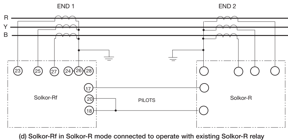
Fig. 6 Connection diagrams (Epsilon case terminal numbers)
