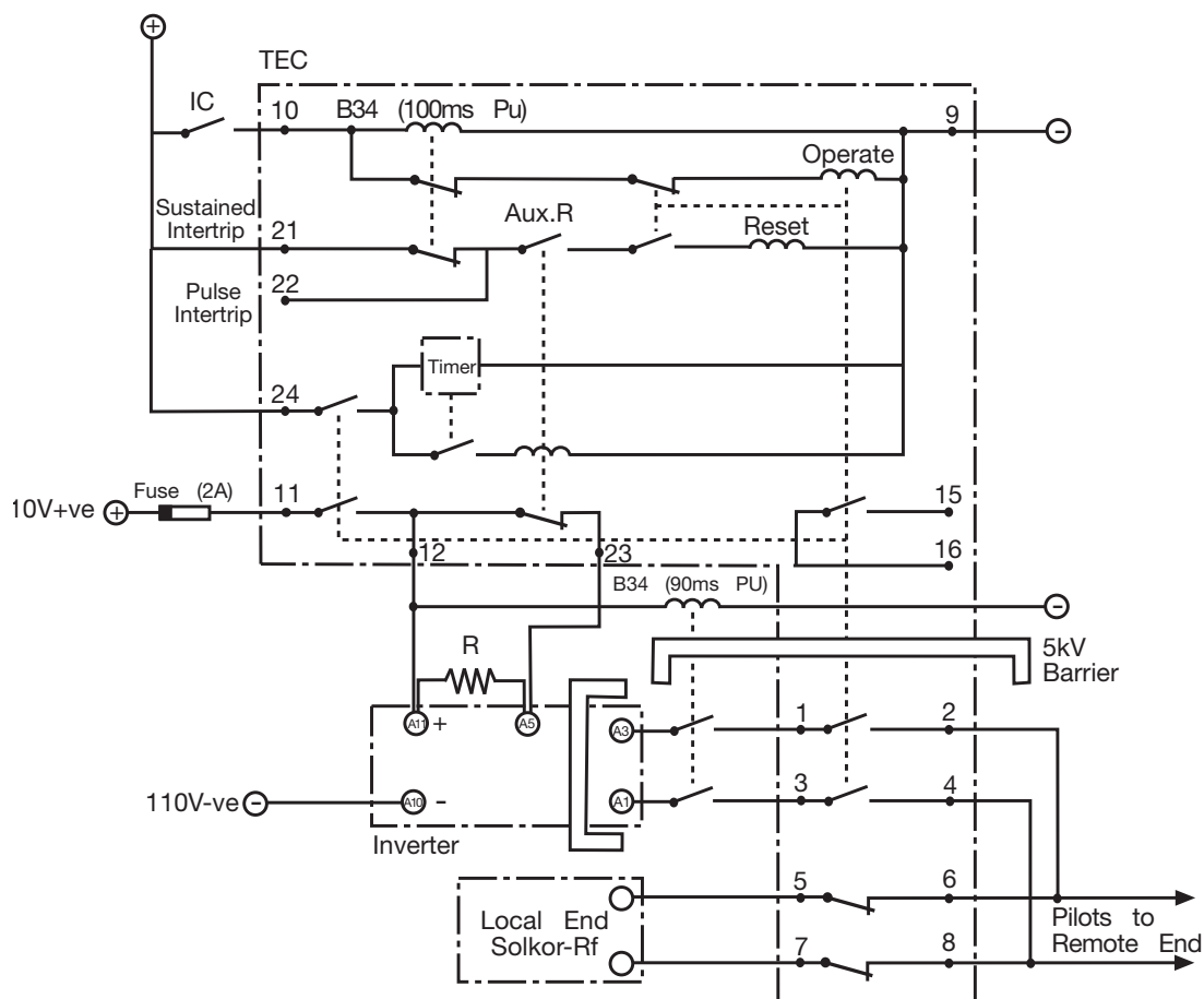
Fig. 9 Typical 2 stage sustained intertripping scheme for Solkor-Rf. send end.
