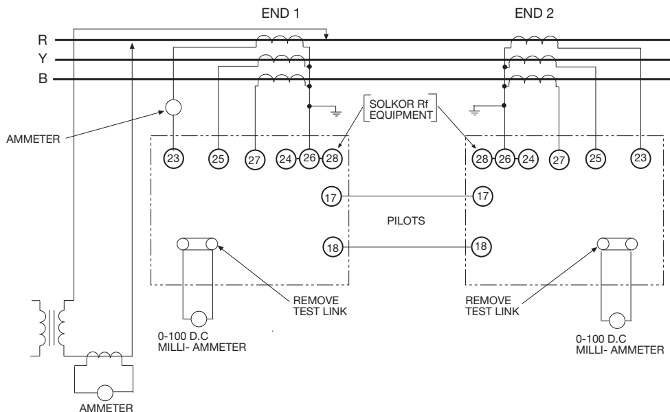
Fig. 2 Connections for overall fault setting tests by primary injection
