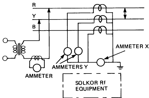
Fig. 1(a) Phase to phase injection
