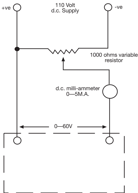
Fig. 7a Secondary injection test of pilot supervision receive relay.
