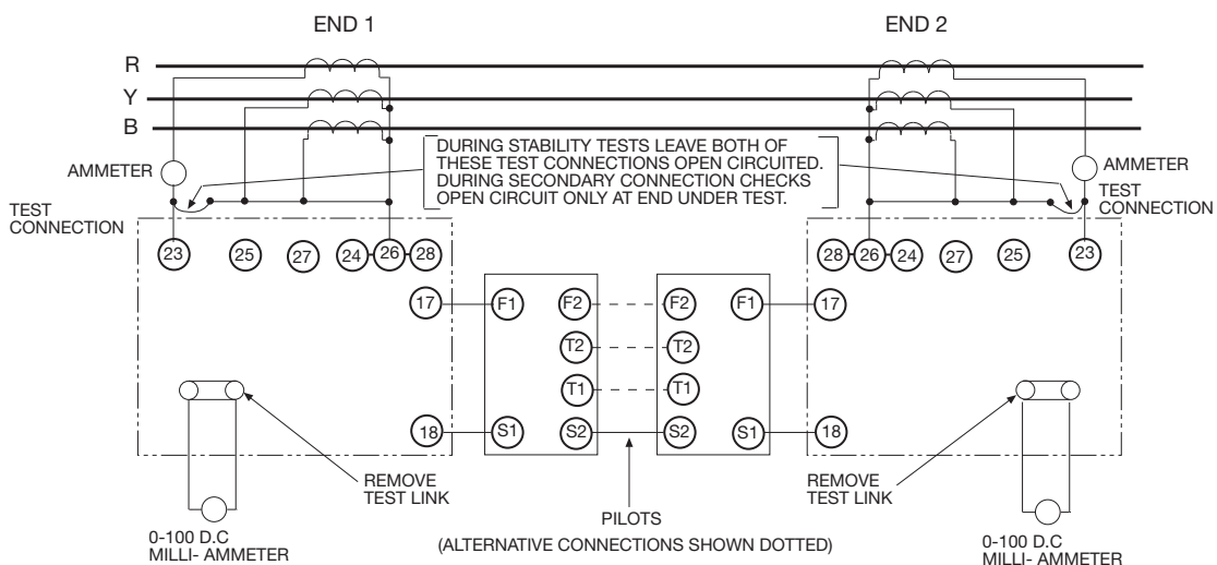
Fig. 3(b) Connections for stability tests and for check of secondary connections using three phase load current (Solkor-Rf with isolating transformers)
