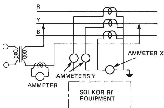
Fig. 1(b) Single phase injection
