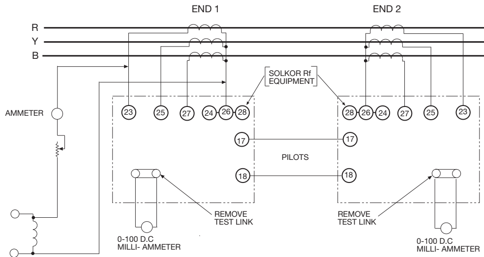
Fig. 4 Connections for overall fault setting tests by secondary injection
