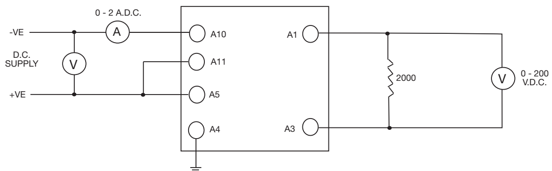
Fig. 10 Test circuit inverter.
