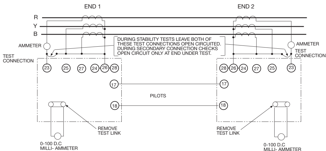
Fig. 3(a) Connections for stability tests and for check of secondary connections using three phase load current (Solkor-Rf without isolating transformers)
