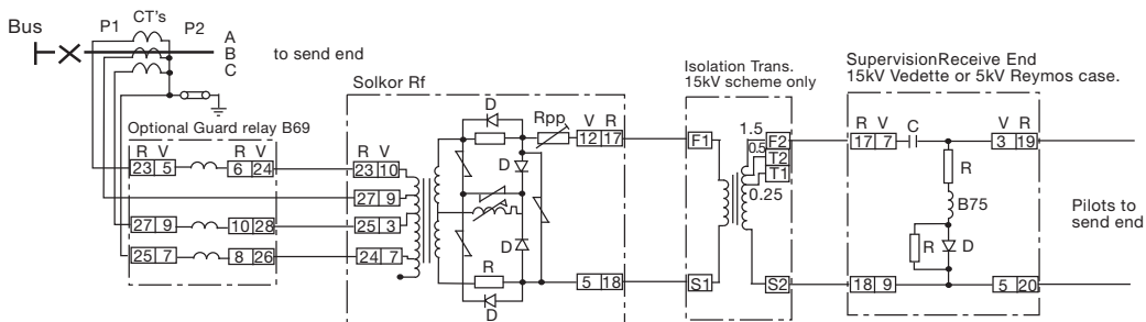
Receive equipment AC schematic diagram
