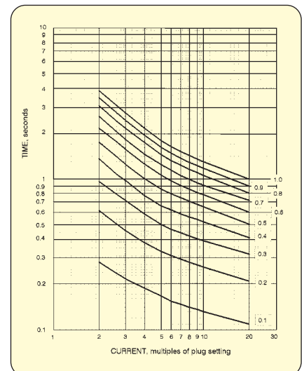
Fig. 1. Time/current characteristic
