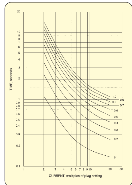
Fig. 1. Time/current characteristic
