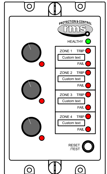
Figure 13: Alarm text position layout
