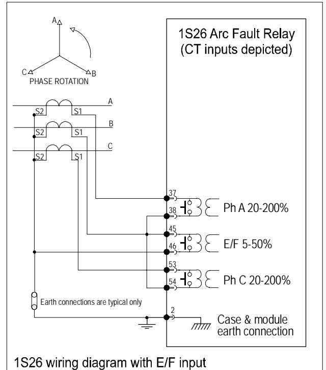
Figure 11: CT wiring configuration when using earth fault input
