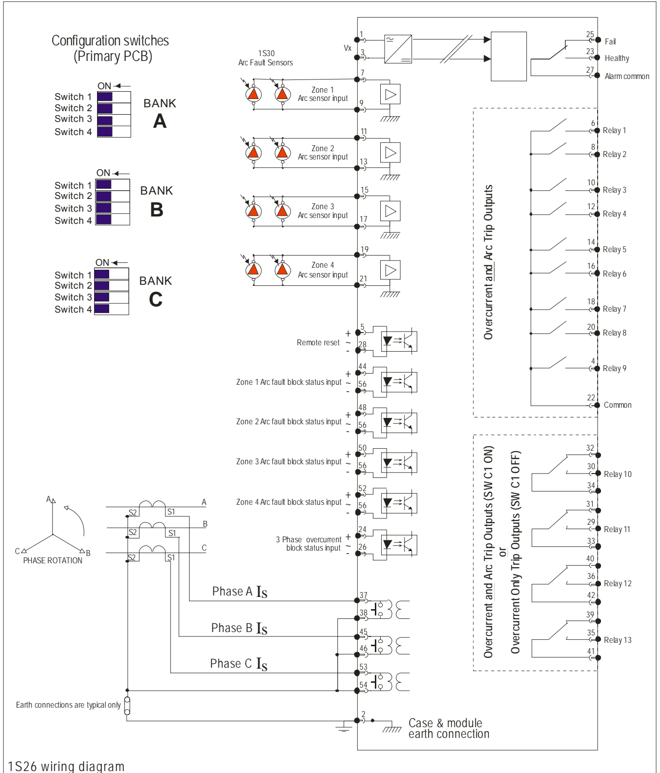
Figure 9: Wiring diagram for 1S26 four zone arc fault monitor - Relays shown in de-energized condition Refer to figure 11 for two phase overcurrent + E/F configuration
