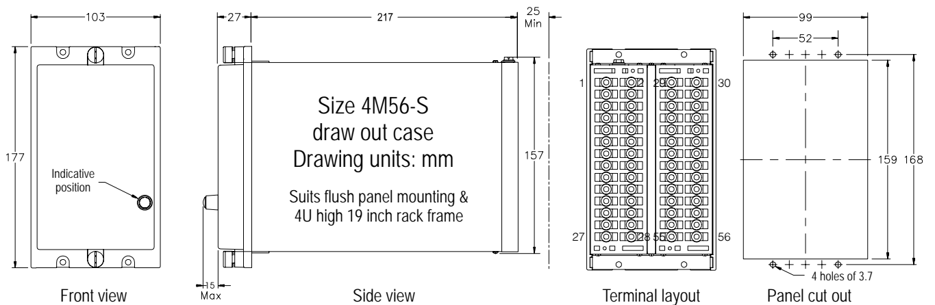
Figure 12: Case mounting details
