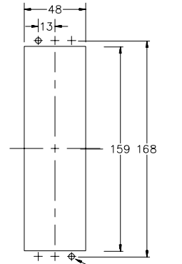
Panel cut out
