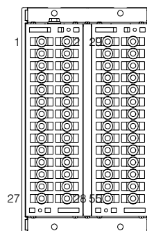
Terminal layout
