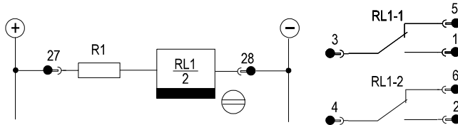
Contacts shown with CB Open & circuit de-energised
