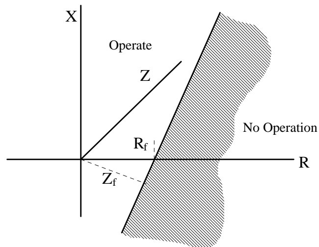
Figure 12 Resistance Characteristic
