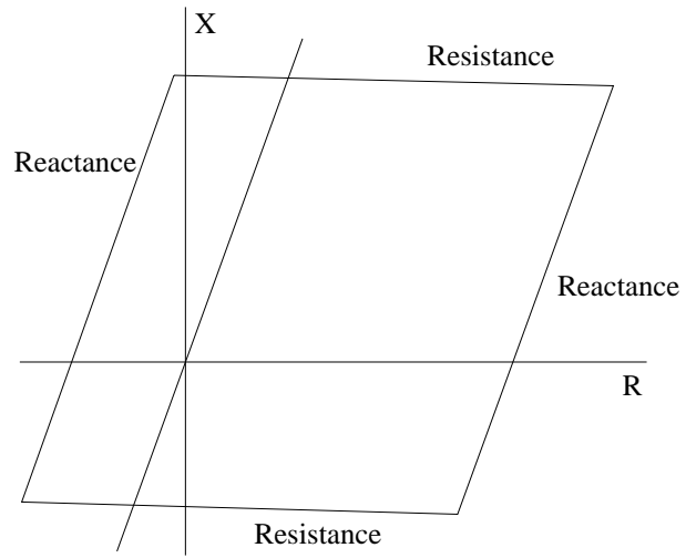
Figure 13 Typical offset quadrilateral distance characteristic
