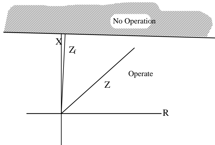
Figure 11 Reactance Characteristic
