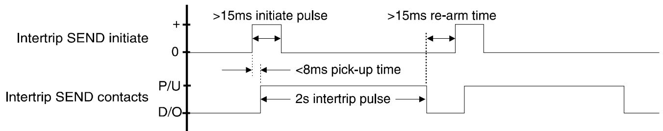
Figure 3: Timing diagram for Intertrip SEND 'pulse' initiate
