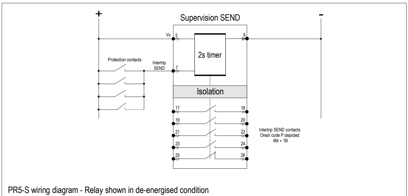
Figure 9: PR5-S application diagram
