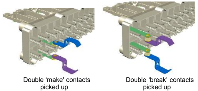
Figure 5: Contact geometry
