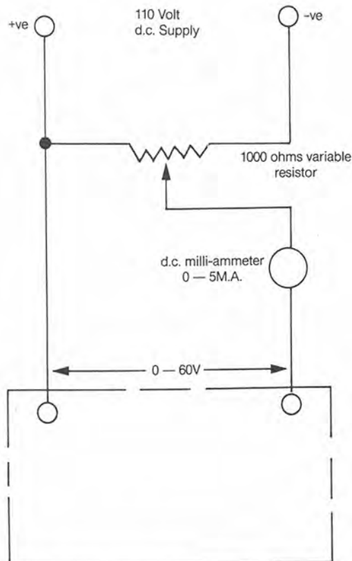
FIG. 1 SECONDARY INJECTION TEST OF PILOT SUPERVISION RECEIVE RELAY
