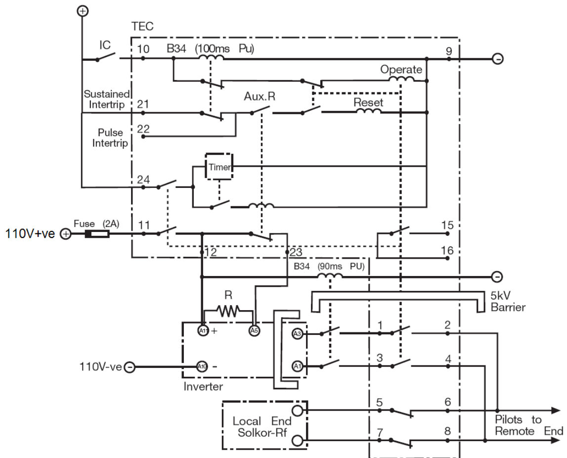
Fig. Typical 2 stage sustained intertripping scheme for Solkor –Rf. Send End.
