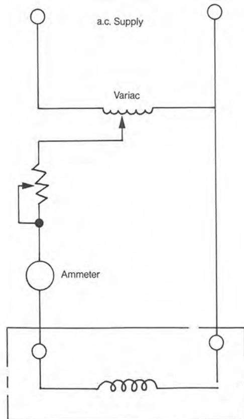
FIG. 2 SECONDARY INJECTION TEST OF GUARD RELAYS. (REFER TO RELEVANT SCHEMATIC FOR TERMINAL NOS.)
