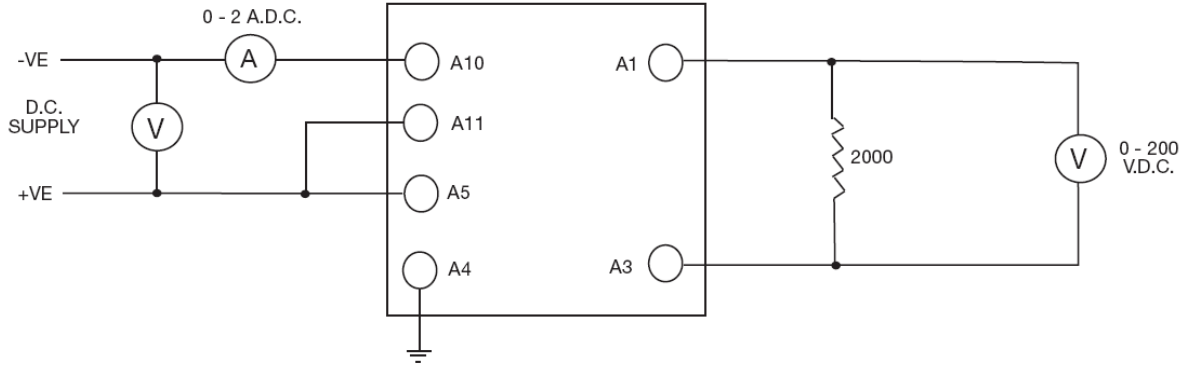
Fig. Test Circuit – Inverter
